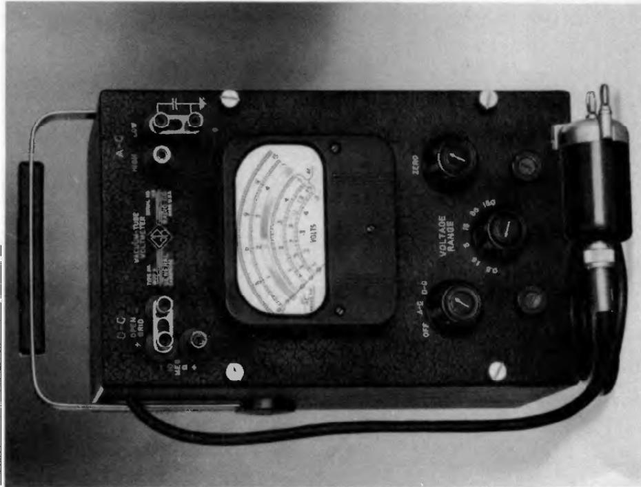
Figure 1. Panel view of the Type 1800-A Vacuum-Tube Voltmeter (left) with handle in vertical carrying position, and (right) with the handle locked in position for supporting instrument with inclined panel.
